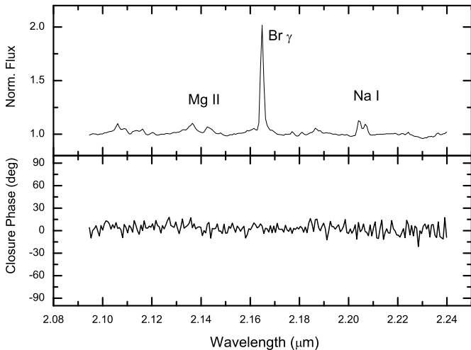
Fig. 4. VLTI/AMBER closure phase for CPD-57° 2874 obtained around Br \gamma with spectral resolution R = 1500 . Within the noise level ( \simeq \pm 10^\circ ) the closure phase is zero both in the continuum and in the Br \gamma line. This strongly suggests that the CSE has an approximately centrally-symmetric projected intensity distribution in the near-IR.
