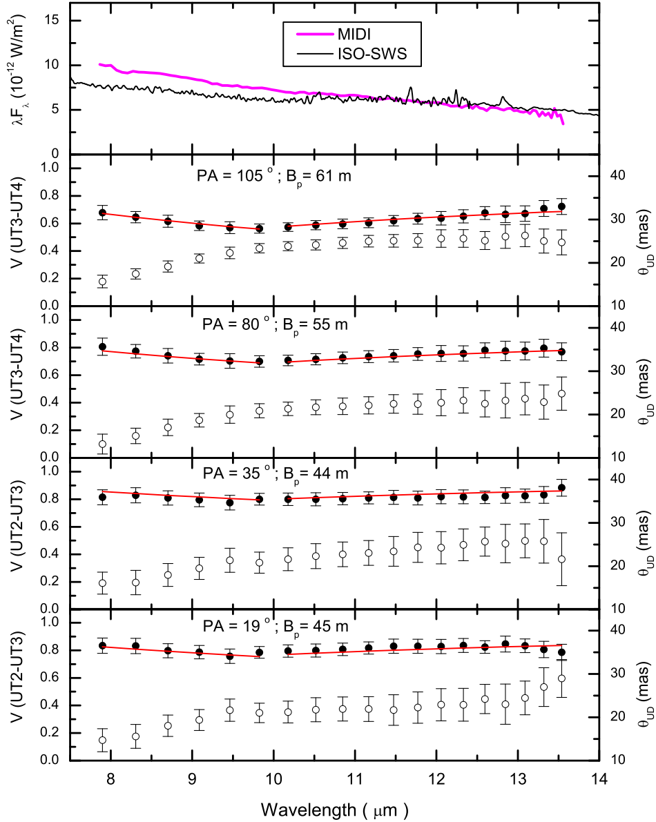
Fig. 3. VLTI/MIDI observations of CPD-57° 2874 obtained in the mid-IR with spectral resolution R = 30 . This figure is organized as Fig. 2, but here V and \theta_{UD} are shown as filled and open circles, respectively. The MIDI and ISO-SWS (Sloan et al. 2003) spectra (top panel) do not show any clear evidence of a silicate feature around 10 \mu\text{m} . The MIDI visibilities are well fitted with an elliptical Gaussian model (solid lines; Eqs. 1 and 2, and Table 4).
